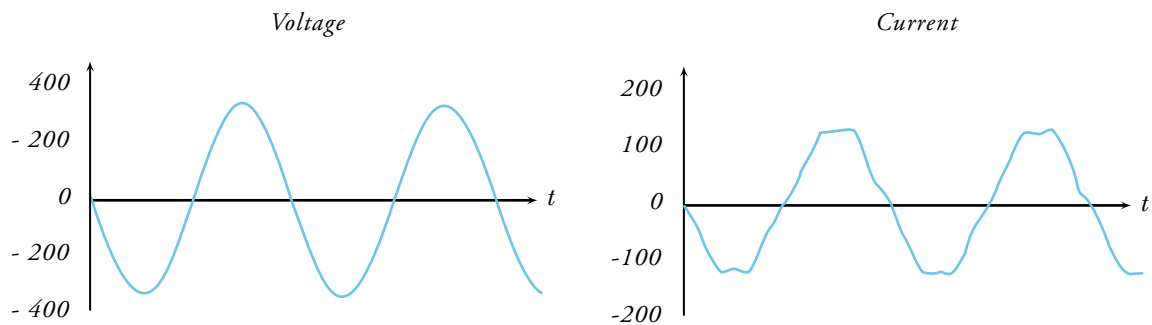
Mains supply voltage and current with an APR, THVD: 1%, THID: 6%
