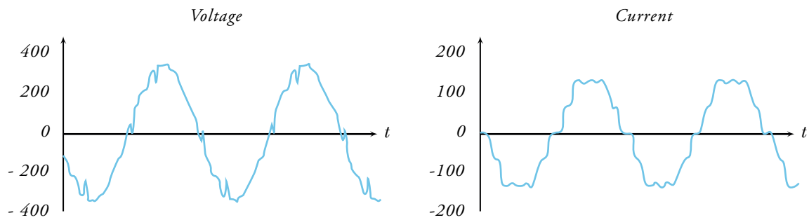
Mains supply voltage and current without an APR, THVD: 8%, THID: 11%
