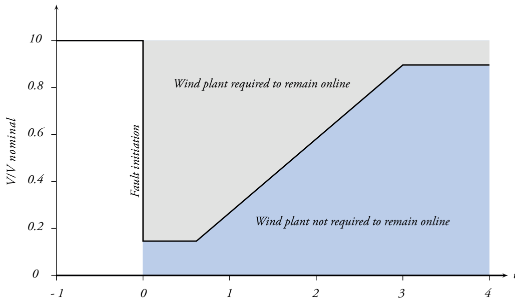
Minimum required wind plant response to emergency low voltage, FERC
