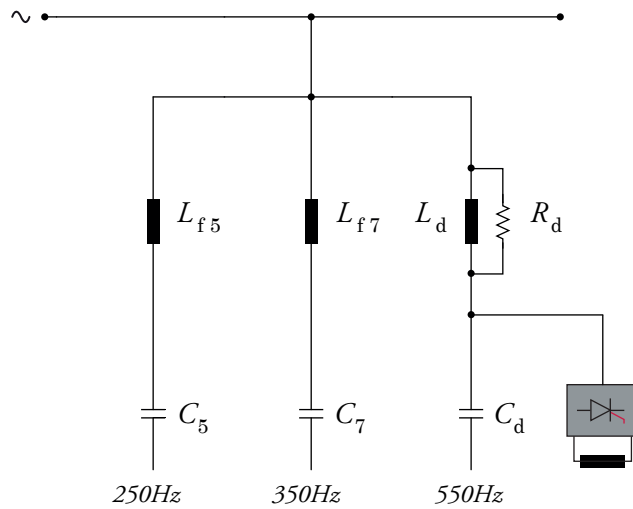
Fig. 8b - Single phase equivalent representation of APR circuit - multiple tuned branches plus a damped branch
