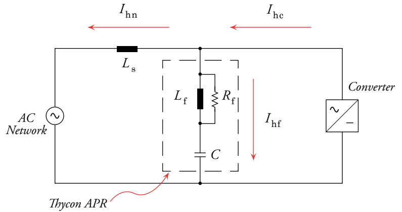
Fig. 9b - Circuit for compensation of harmonic currents on the AC side of a converter.
