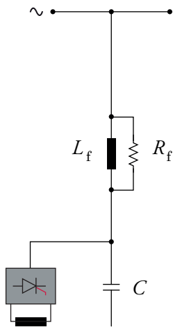
Fig. 8a - Single phase equivalent representation of APR circuit - a single damped branch
