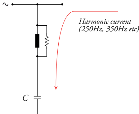
Fig. 9a - Single phase equivalent representation of APR circuit for harmonic analysis
